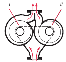
Both pumps operating
