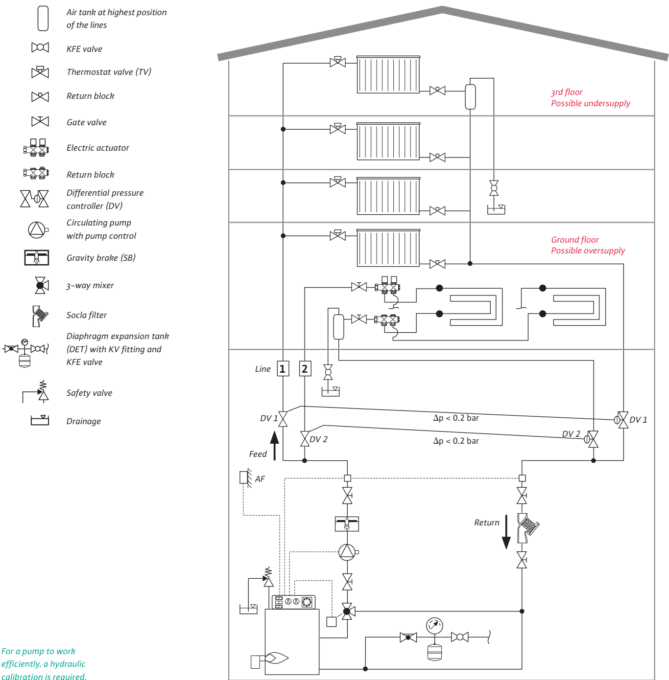
Schematic diagram of a heating system with a facility for hydraulic calibration
