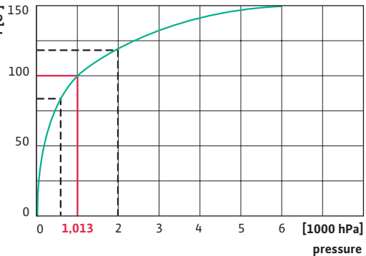
Boiling point of water as a function of pressure
