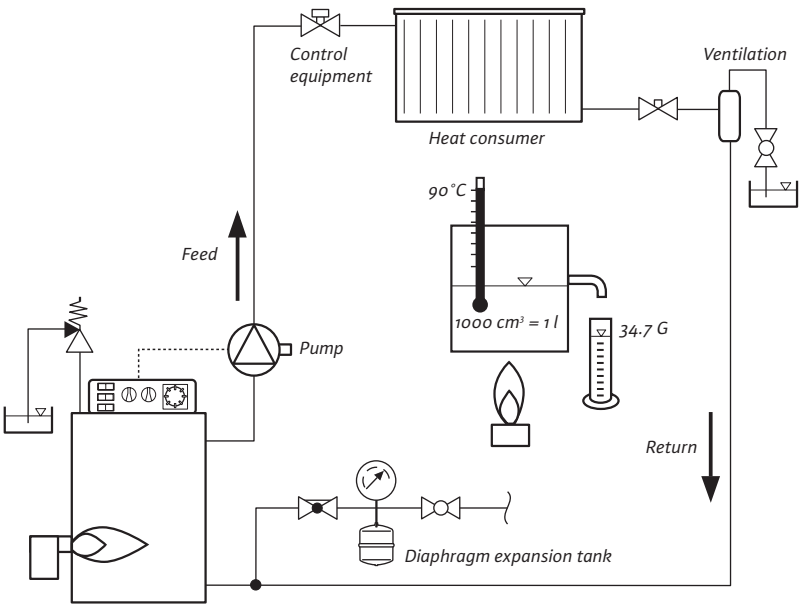
Illustration of a heating system with integrated safety valve
