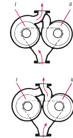
Pump I or pump II operating
