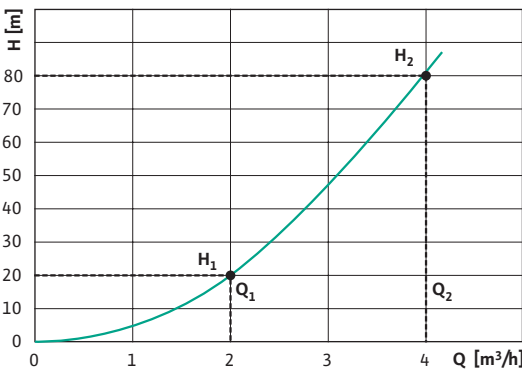
System curve
