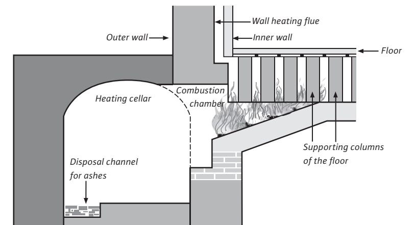
Illustration of a hypocaust heating system from Roman times
