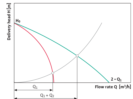
Both pumps operating
