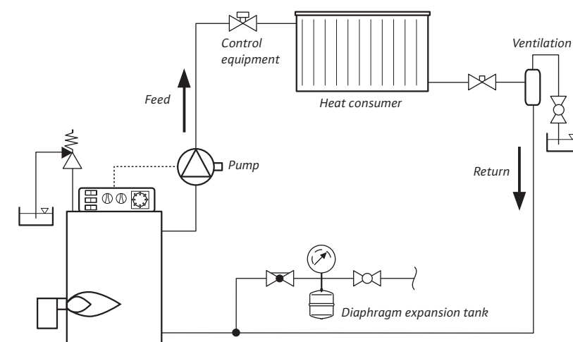
Circulating system using the example of a heating system
