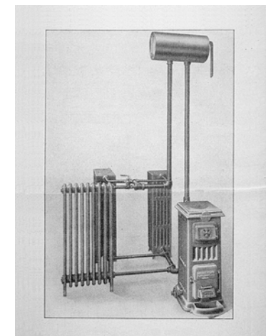
Gravitational heating system with boiler, expansion tank and radiator
