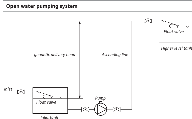
Pump system for pumping water to a higher level
